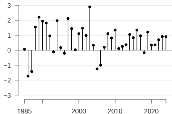
Raw residuals (deviances)
