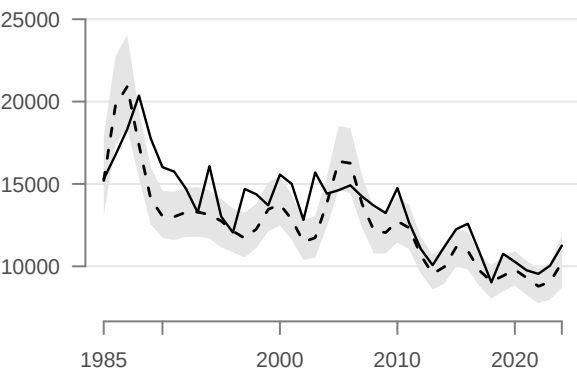
Prediction error
