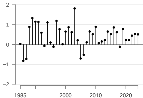
Standardized residuals
