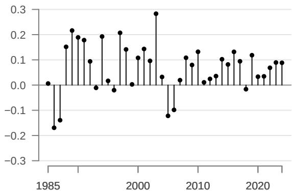
Raw residuals (deviances)
