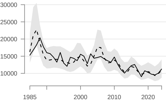
Prediction error
